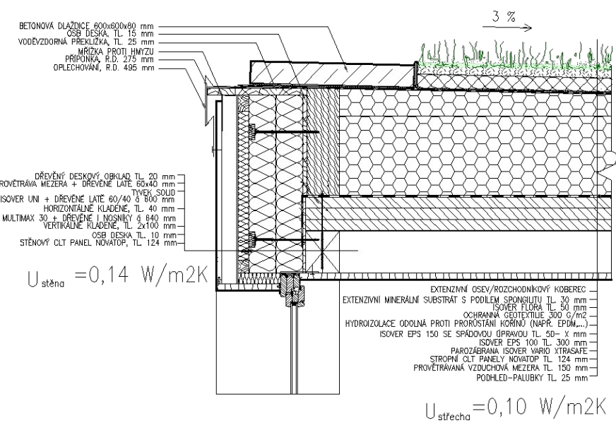
DETAIL B 1:20
