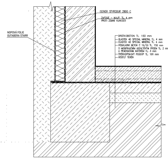
DETAIL A 1:20
