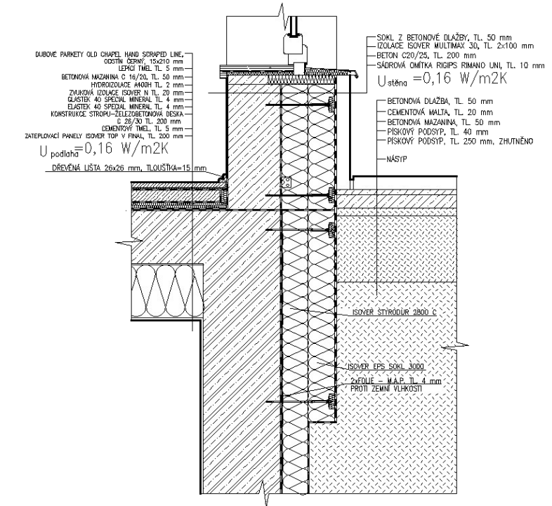
DETAIL D 1:20
