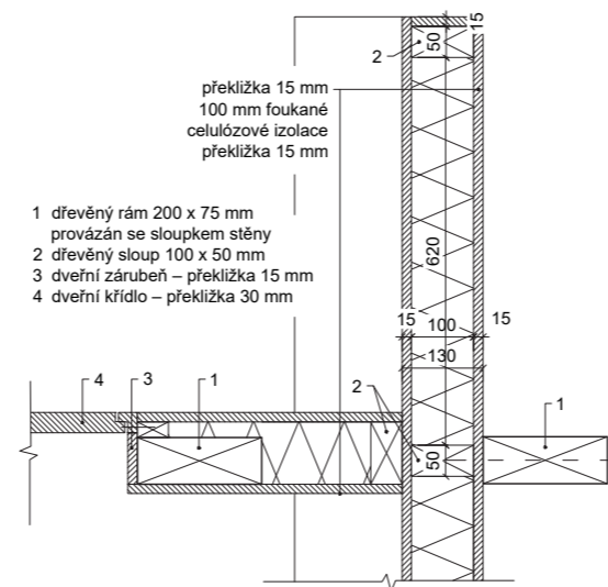
Detail E 1:20
