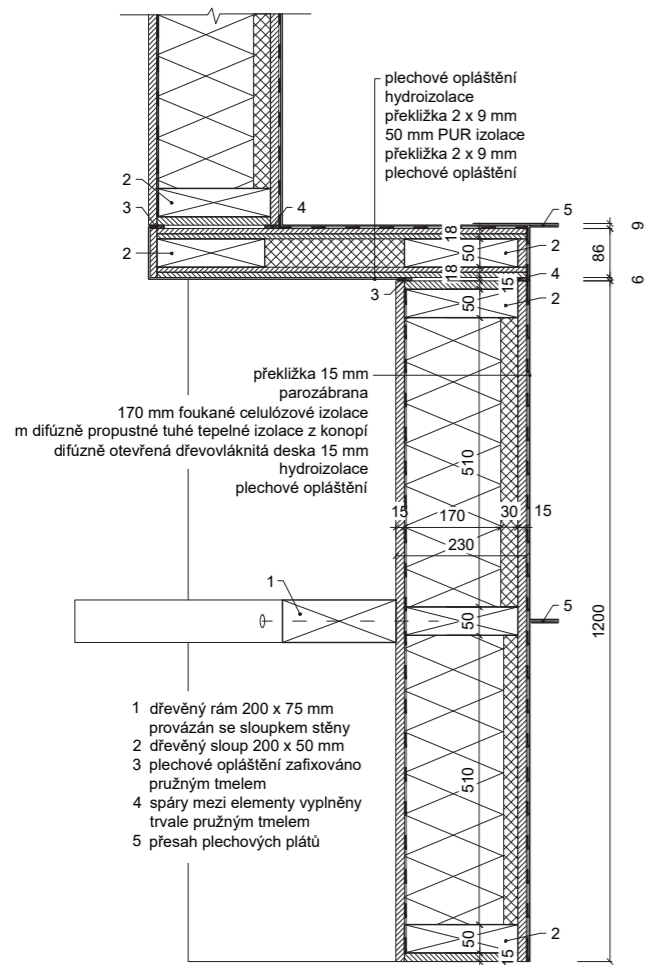
Detail A 1:20
