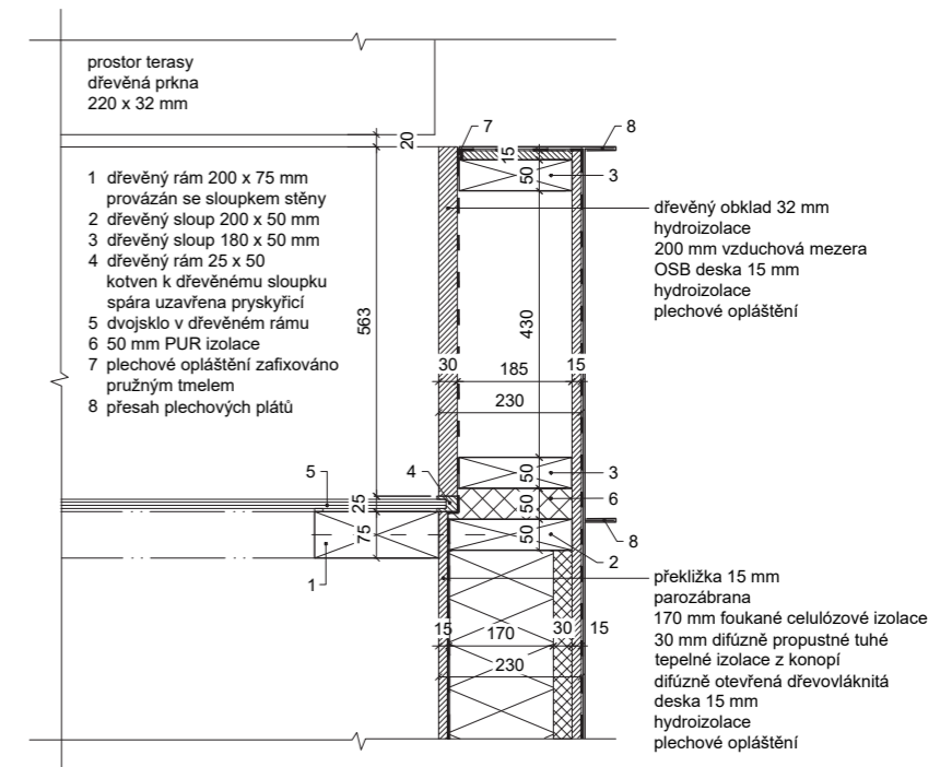
Detail C 1:20
