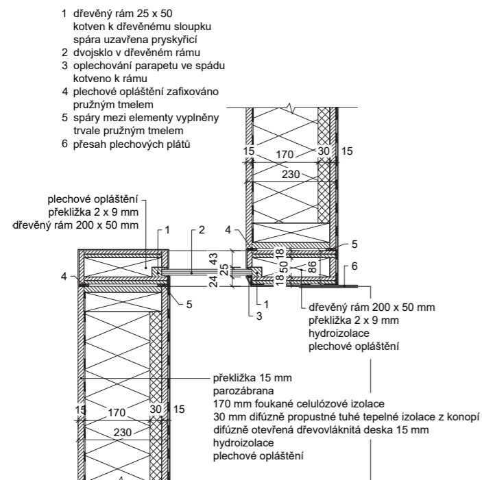
Detail D 1:20
