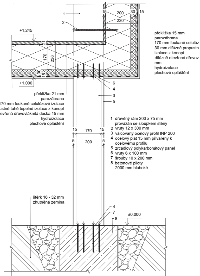
Detail B 1:20
