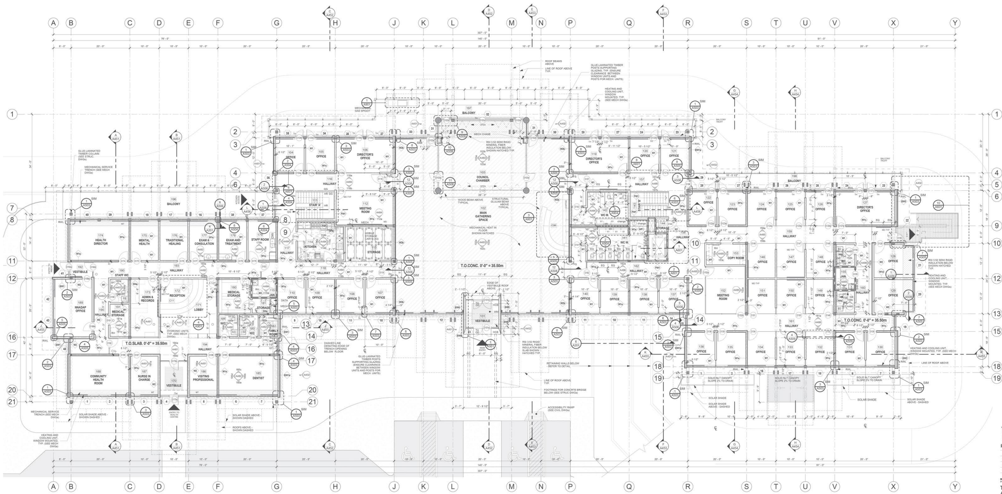
A MAIN FLOOR PLAN 1/8" = 1'-0"
